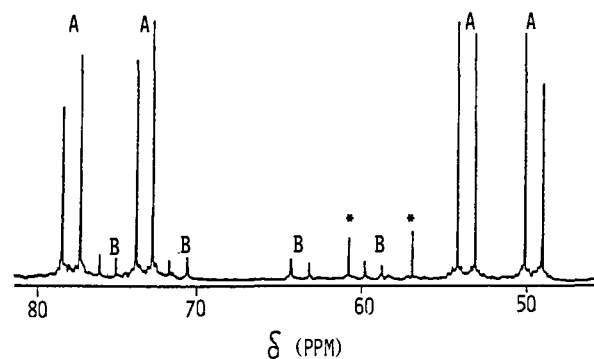
Figure 3. ^{31}\text{P}\{^1\text{H}\} NMR spectra of [\text{Rh}(\text{dipamp})(\text{mac})]^+ ( 2 ) at 29.6 °C: A, major diastereomer ( 2^{\text{maj}} ) \delta_{\text{P}_1} = 51.3 ppm, J_{\text{P}_1-\text{Rh}} = 150 Hz, J_{\text{P}_1-\text{P}_2} = 39.5 Hz; \delta_{\text{P}_2} = 74.7 ppm, J_{\text{P}_2-\text{Rh}} = 162 Hz. B, minor diastereomer ( 2^{\text{min}} ) \delta_{\text{P}_1} = 60.5 ppm, J_{\text{P}_1-\text{Rh}} = 167 Hz, J_{\text{P}_1-\text{P}_2} = 36.5 Hz; \delta_{\text{P}_2} = 72.7 ppm, J_{\text{P}_2-\text{Rh}} = 160.5 Hz. * = [\text{Rh}(\text{dipamp})_2]^+ impurity ( \text{P}_1 is trans to \text{O}=\text{C} ; \text{P}_2 is trans to \text{C}=\text{C} ).
