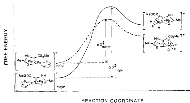
Figure 9. Schematic reaction coordinate profiles for the enantio-determining reactions of the diastereomeric [Rh(dipamp)(mac)] + adducts with H 2 .
